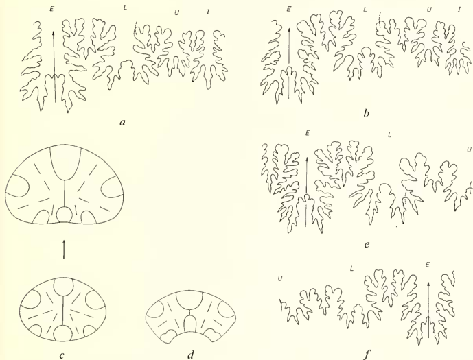
TEXT-FIG. 1. Eoscaphtes , suture and whorl sections. a-c : E. circularis (J. de C. Sowerby). a , Complete suture of the ammonitid coiled hypotype MGL 12341/1; Upper Albian, Perte du Rhône. h = 3.5 mm. b , Suture of the crioceratitid uncoiled specimen, GPIT Ce 1221/1; Upper Albian, Folkestone. h = 5 mm. c , Development of whorl section, and hamitid septal surface; the same, \times 4 . d-f , E. subcircularis (Spath). d , whorl section and subsaphitid septal surface, MGL 12342; Upper Albian, Perte du Rhône, \times 2 . e , External suture-line, MGL 12340; same locality. h = 5 mm. f , External suture of the Madagascan hypotype (cf. Collignon 1963, fig. 1144); Upper Albian, Mt. Raynaud. h = 4 mm.
